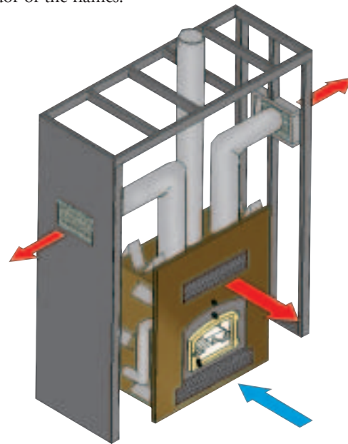
OPTIONAL SIDE HEAT VENTS
